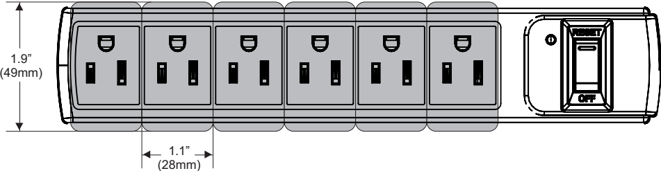
TEC600C,601C: 6-Outlet Power Bar
